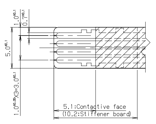
Conductive Face (導通面) FFC-Type Cable
