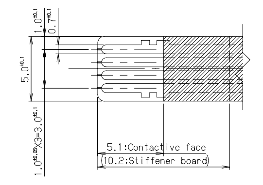
Conductive Face (導通面) FPC-Type Cable
