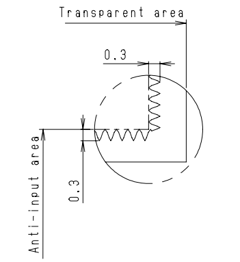
A section enlargement
