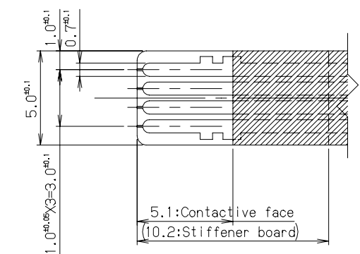
Conductive Face (導通面) FPC-Type Cable
